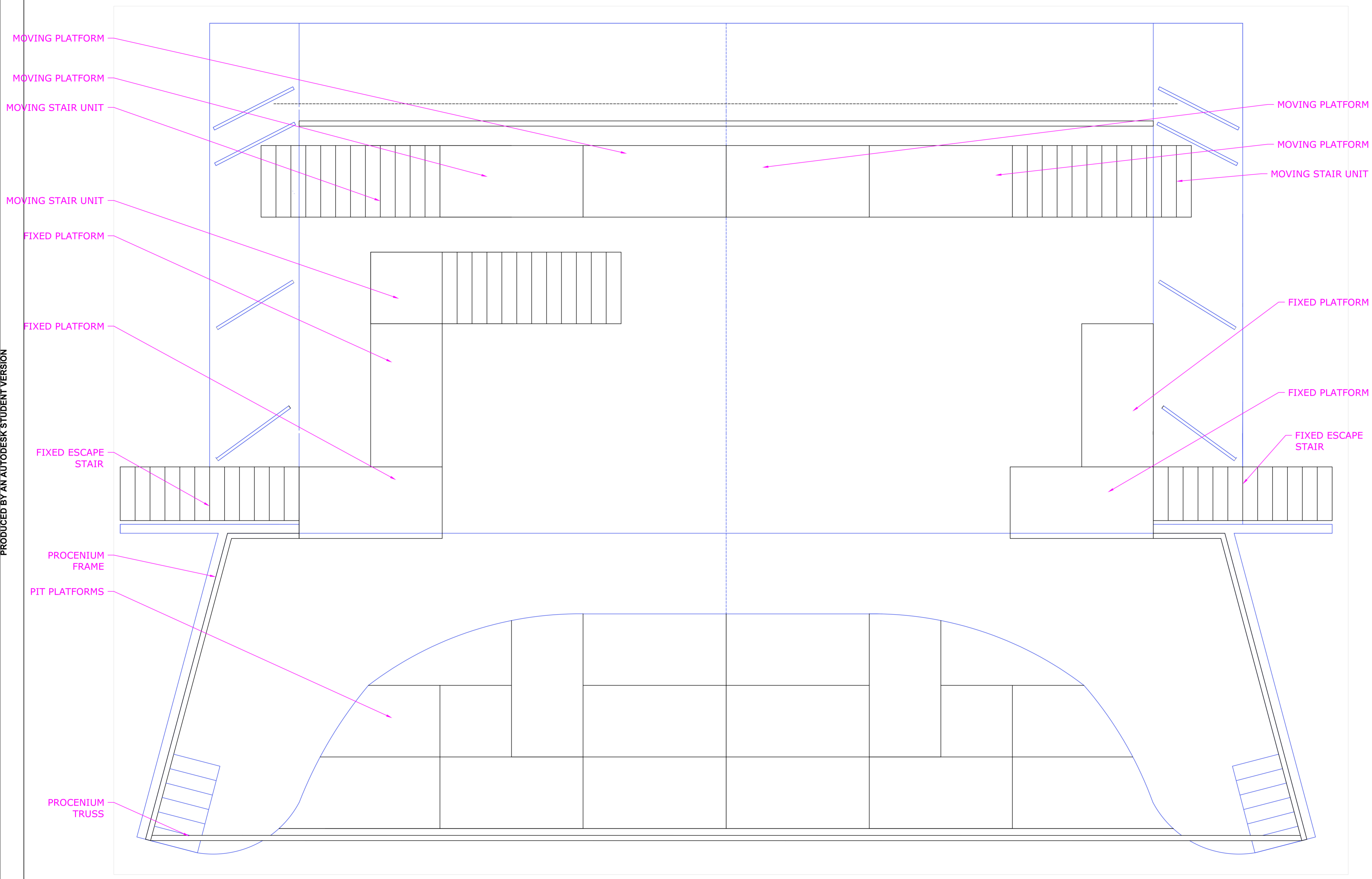
1 GROUND PLAN SCALE: 3/8" = 1'-0" 0 6' 1 2 4
